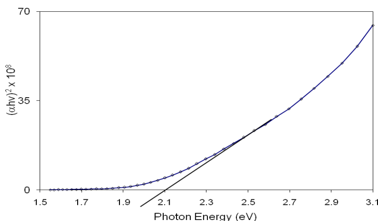
Fig 5: Estimation of optical energy of cadmium selenide thin film.
