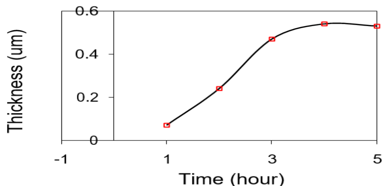
Fig1: Plot of thickness in opposition to deposition time of cadmium selenide.
