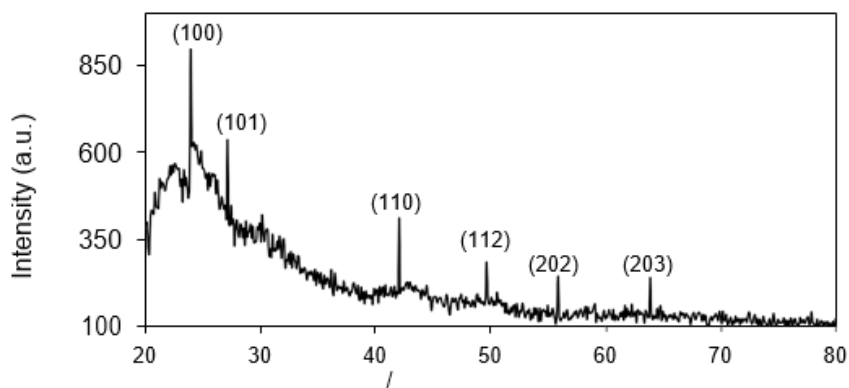
Fig.2: X-ray diffractogram of cadmium selenide sample.
