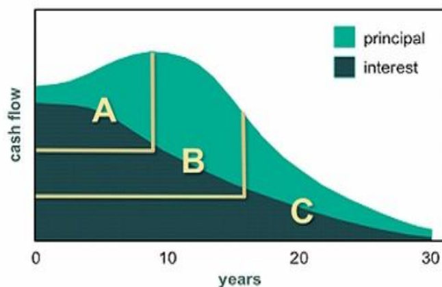
Figure 3:CMO
