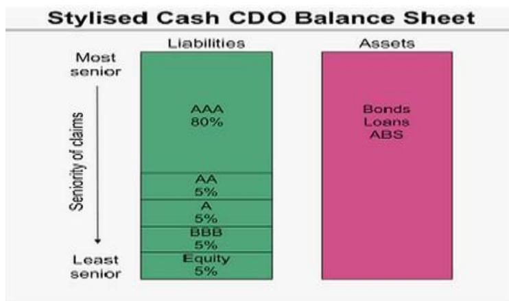
Figure 4: CDO
